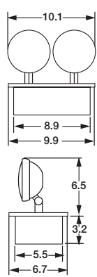
Round Heads Suffix "-R"
